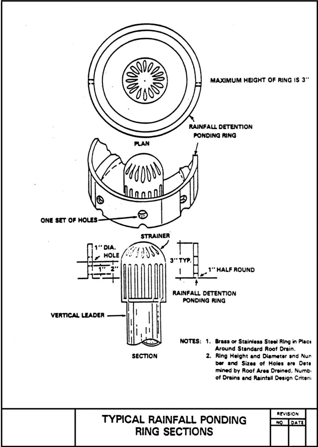
Figure I.2 Typical rainfall ponding ring sections.
